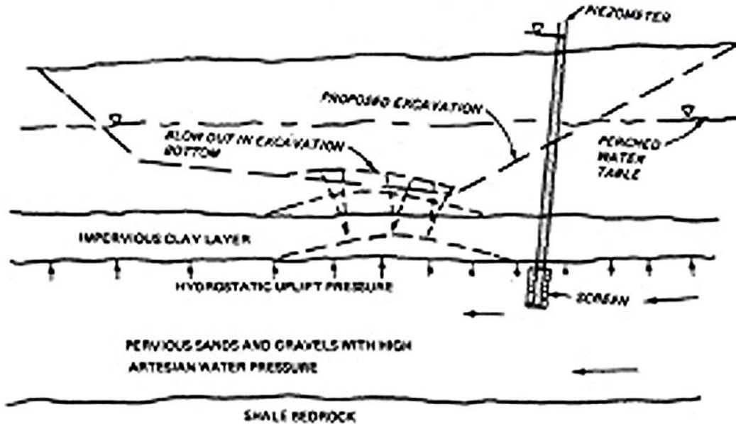
Figure 3-2 Excavation Subject to Bottom Heave
